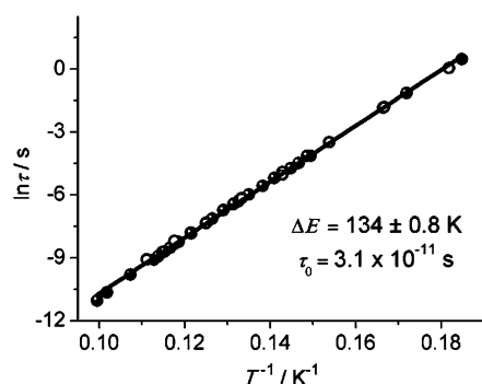
Figure 5. Arrhenius plot displaying T-dependence of the relaxation times for 2 . Open circles indicate that the corresponding relaxation time was extracted from fitting the frequency-dependent AC susceptibility curves with a modified Debye model (see the Supporting Information), whereas the dots indicate that the temperature corresponding to the peak maximum in AC curves was measured at constant frequency.
