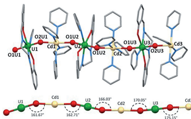
Figure 1. Mercury view of the structure of 1 (top) and a detail of the core with associated distances and angles (bottom). Hydrogen atoms and cocrystallized solvent molecules omitted for clarity. C grey, O red, Cd cream, N light blue, U green.
